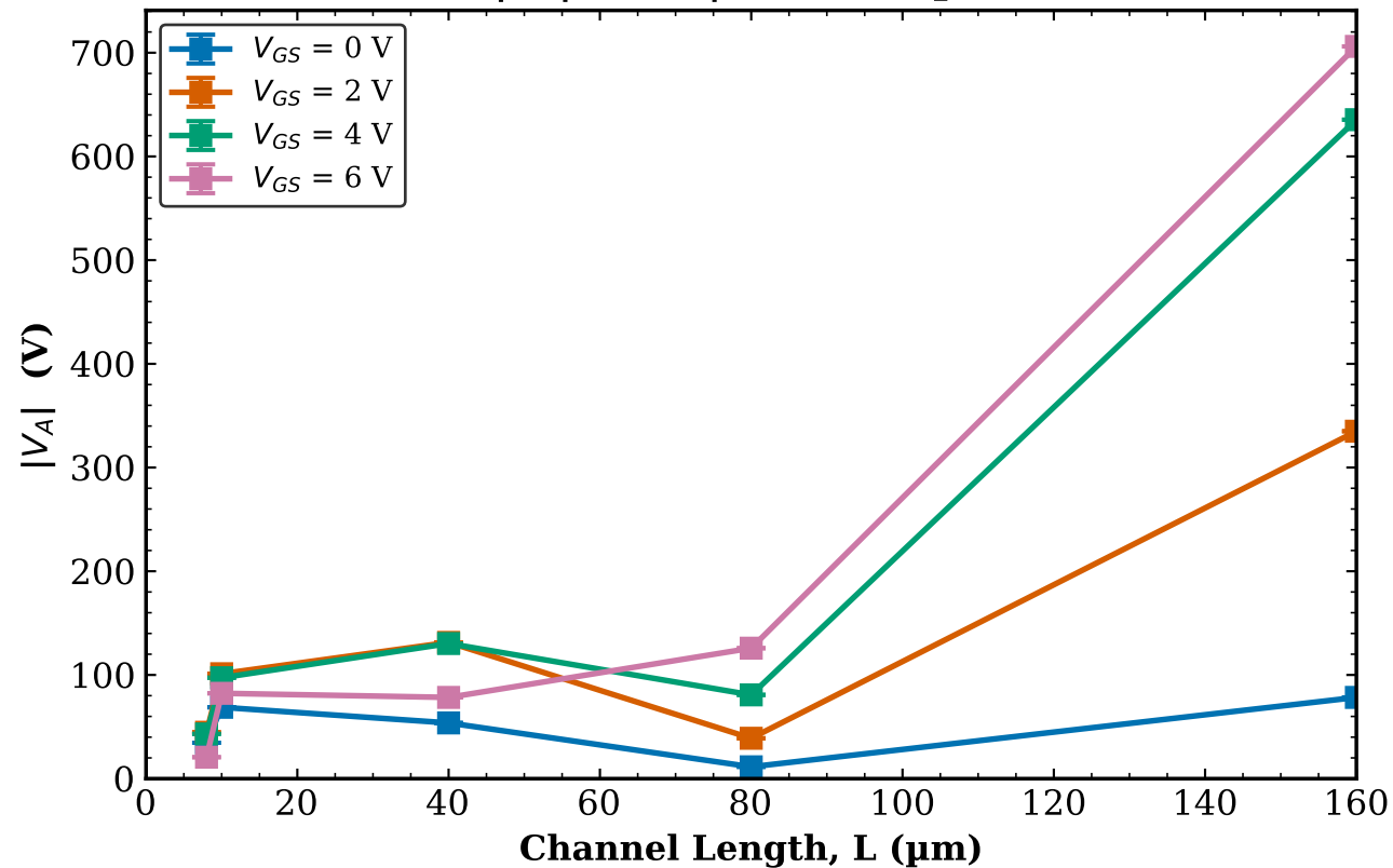
TFT1 Transistor 1 |V_A| vs L | W = 50\text{ }\mu\text{m}
